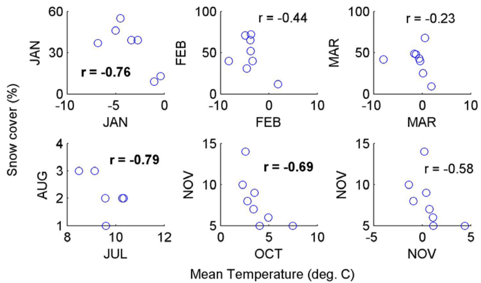
Fig. S2 Correlations between monthly snow cover (%) at 3000-4000 m elevation zone and monthly temperature at the Langtang station at elevation 3920 m. The r values in bold are significant at 5% confidence level.
