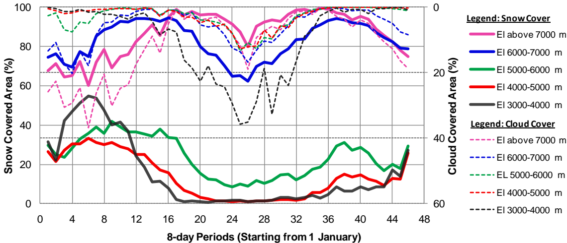
Fig. 2 Variations of the snow cover expressed in percentage of the total area at given 8-day periods of the year in various elevation zones. The values are averages of 9 consecutive years from 2000-2008.
