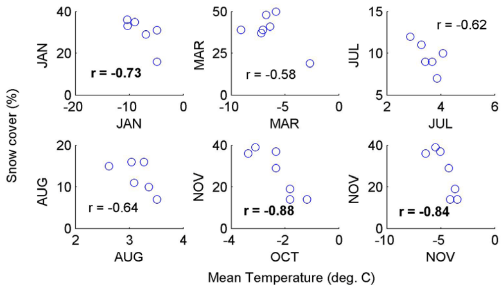
Fig. S1 Correlations between monthly snow cover (%) at 5000-6000 m elevation zone and monthly temperature at the Pyramid station at elevation 5035 m. The r values in bold are significant at 5% confidence level.
