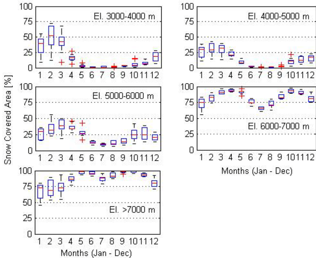
Fig. 3 Monthly variations of snow cover expressed in percentage of total area at various elevation zones presented in box-plots based on 9 years data from 2000 to 2008.
