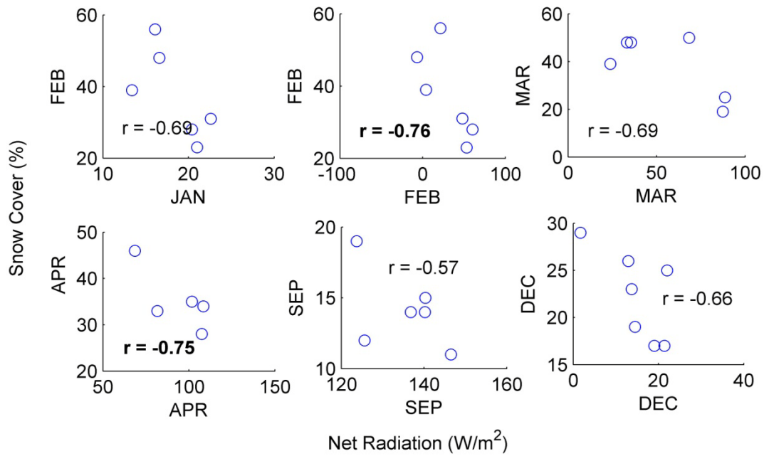
Fig. S3 Correlations between monthly snow cover (%) at 5000-6000 m elevation zone and monthly net radiation at the Pyramid station at elevation 5035 m. The r values in bold are significant at 5% confidence level.
