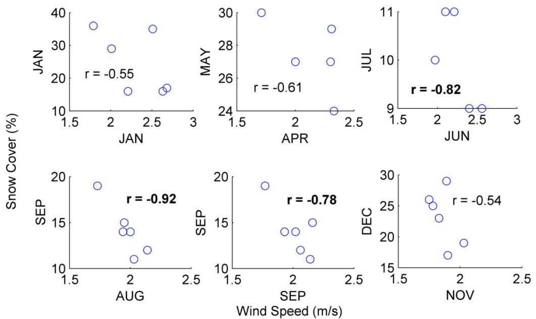
Fig. S4 Correlations between monthly snow cover (%) at 5000-6000 m elevation zone and monthly wind speed at the Pyramid station at elevation 5035 m. The r values in bold are significant at 5% confidence level.
