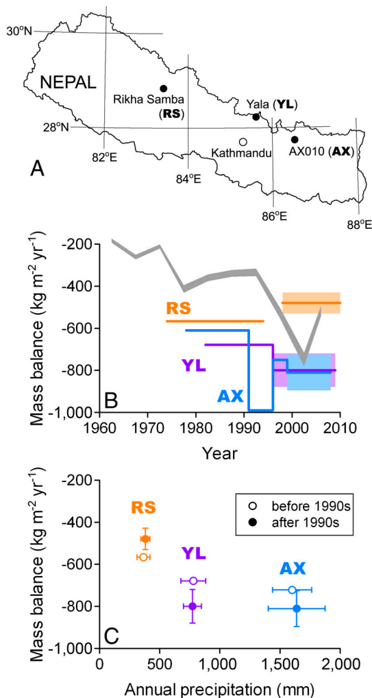
Fig. 1. Location of the three benchmark glaciers in Nepal (A), temporal changes in the area-averaged mass balances of the glaciers compared with the pentadal global mean (gray line) (6) (B), and mass balances compared with annual precipitation (C). Color shading in B and vertical bars in C denote measurement errors of mass balance. Horizontal bars in C denote variability of annual precipitation. See SI Text about the error evaluation and the downscaling.
